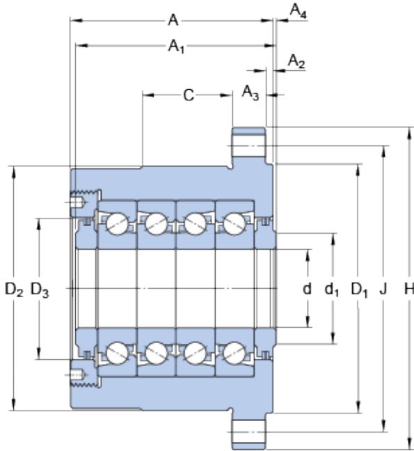
FBSA 206 A/QBC Bearing 2D drawings and 3D CAD models
